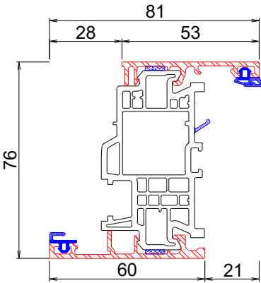
Anta standard
