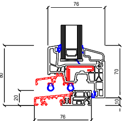
Anta Slim
