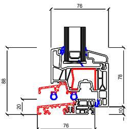
Anta Standard
